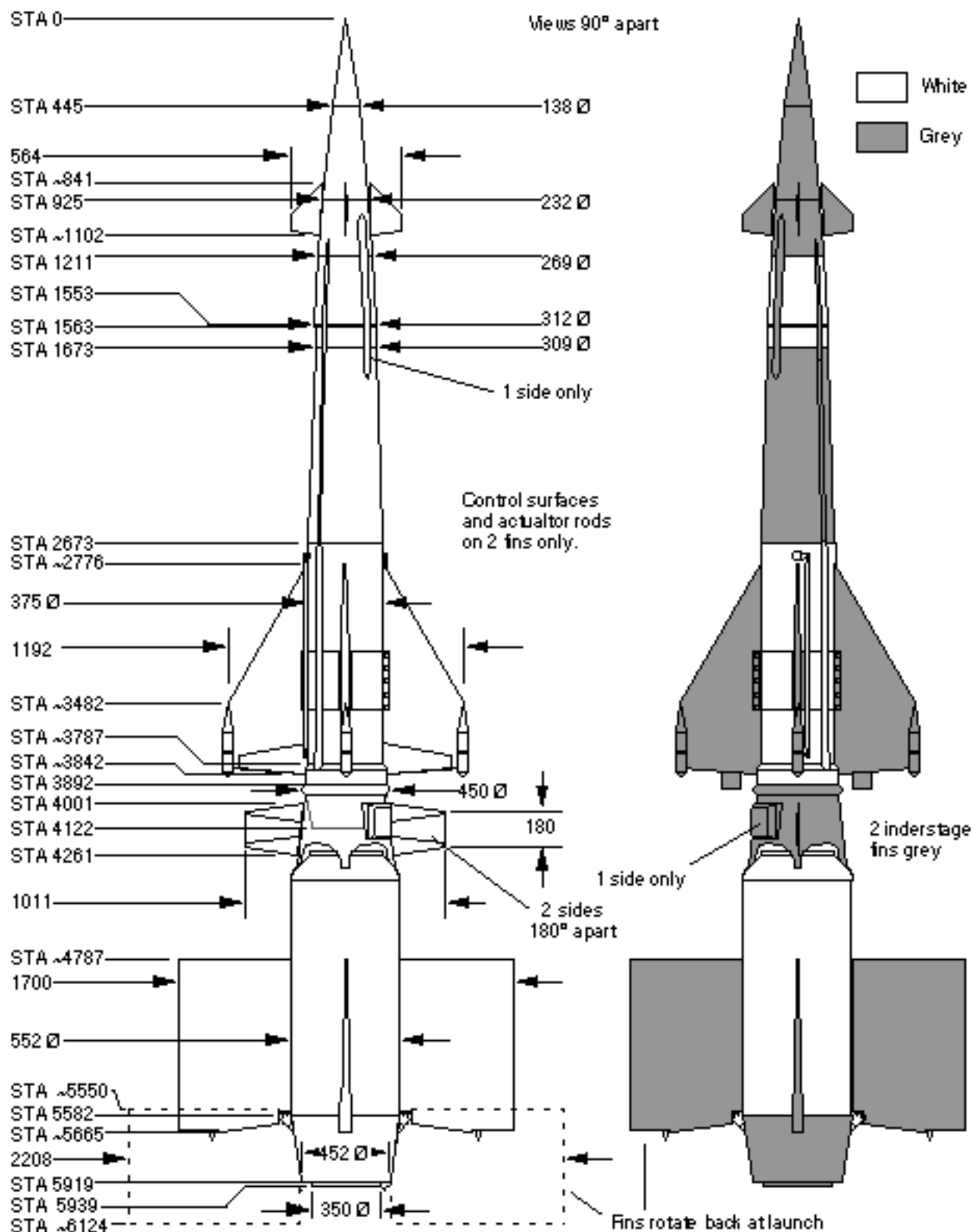
Lavochkin S-125 Neva SA-3B Goa 1/30 scale Dimensions in millimeters
