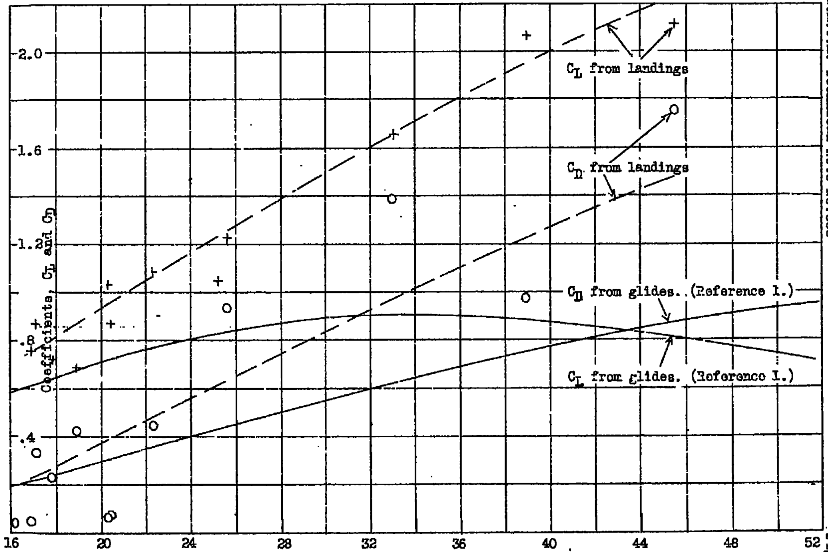
Figure 3.-Lift and drag coefficients of a PCA-2 autogyro.
