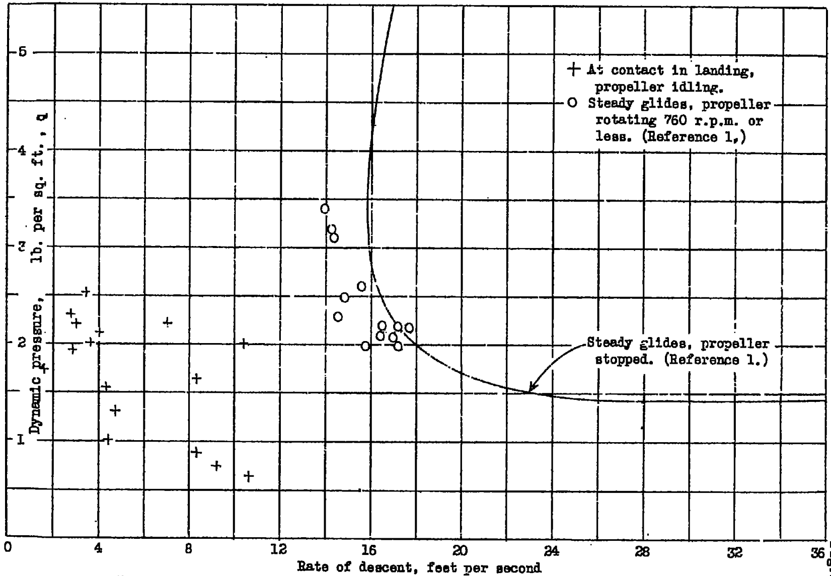
Figure 1.-Variation of rate of descent of a PGA-2 autogyro with dynamic pressure.
